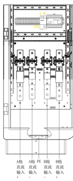
风冷终端300A/400A双枪
